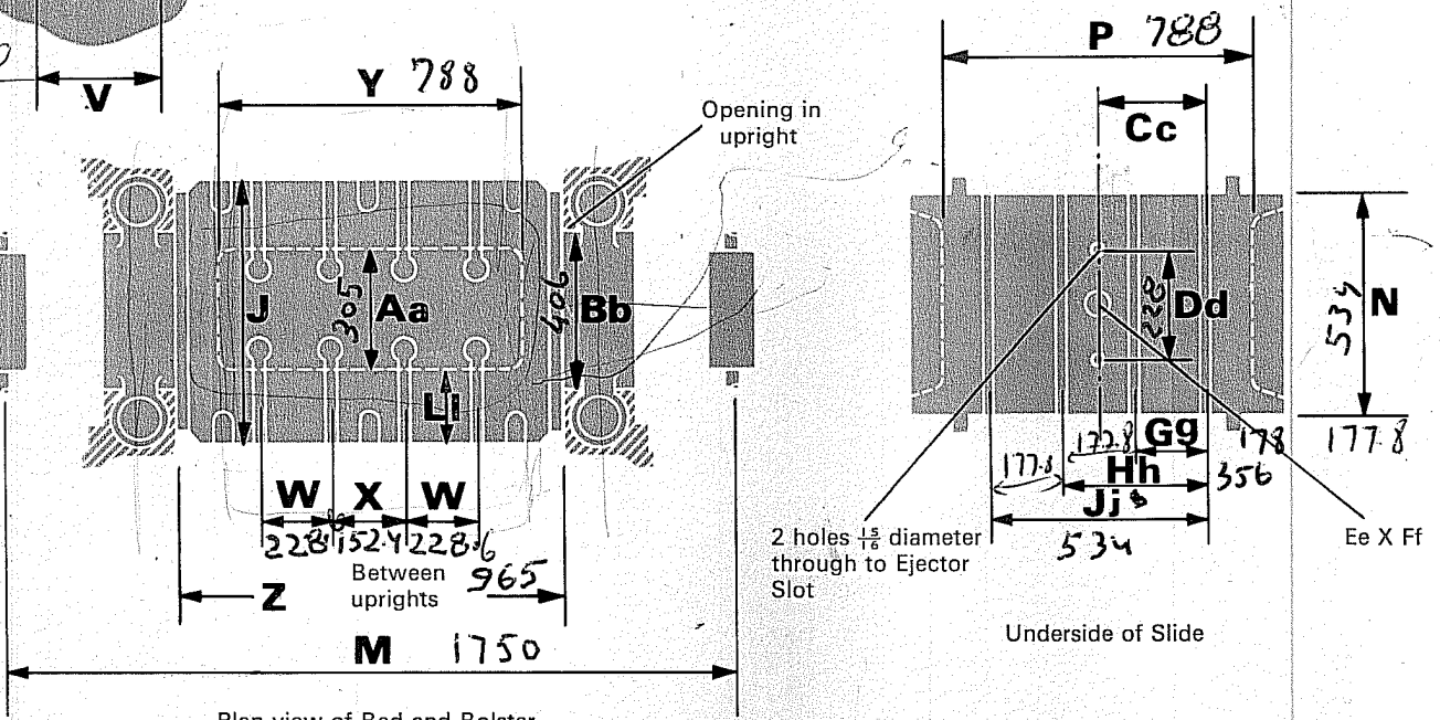
Plan view of Bed and Bolster
